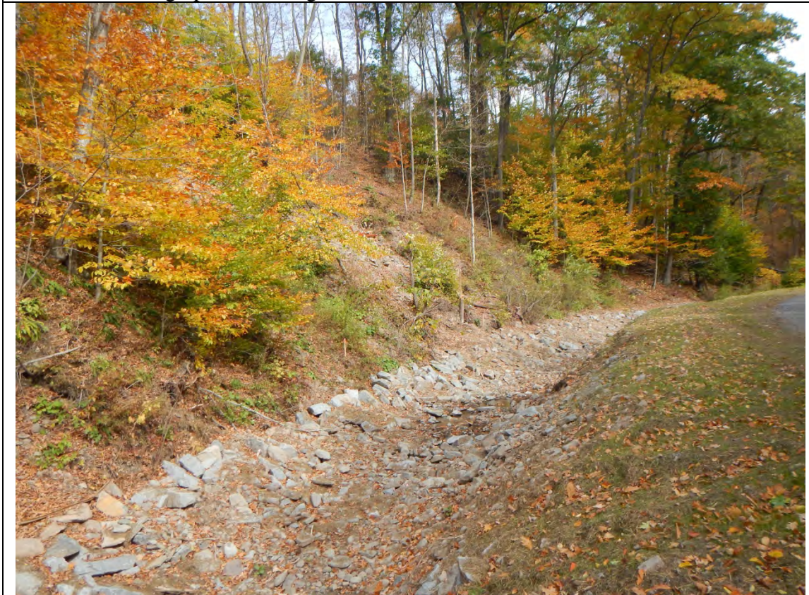
Photo 4: Looking upstream after construction of rock rip rap along the toe of right streambank and a hardened riffle.
